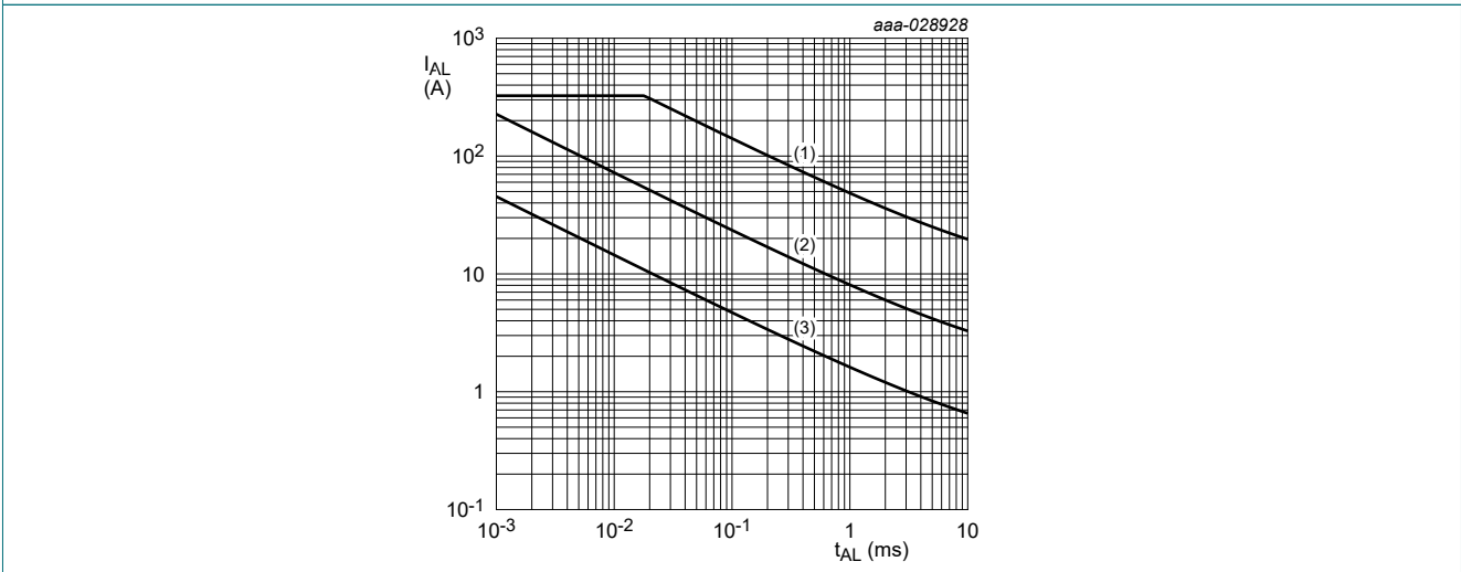
Fig. 4. Peak Current Capability
