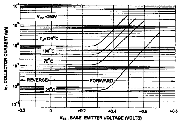
FIG-8 COLLECTOR CUT-OFF REGION
