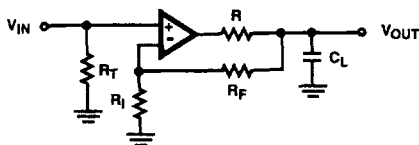
FIGURE 6. PLACEMENT OF THE OUTPUT ISOLATION RESISTOR, R
