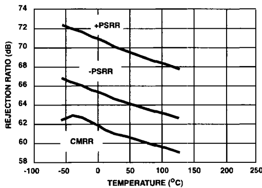
FIGURE 31. REJECTION RATIO vs TEMPERATURE
