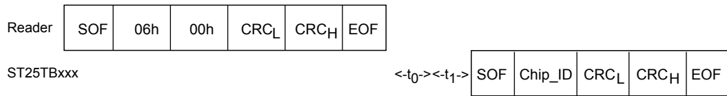
Figure 47. Initiate frame exchange between reader and ST25TB04K
