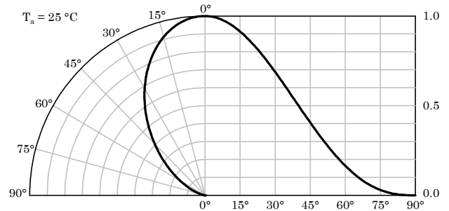
Spatial Distribution
