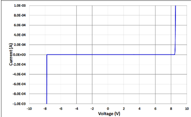
Figure 6-5. IV Curve
