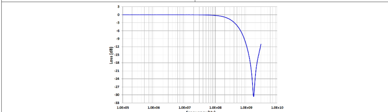
Figure 6-9. Insertion Loss
