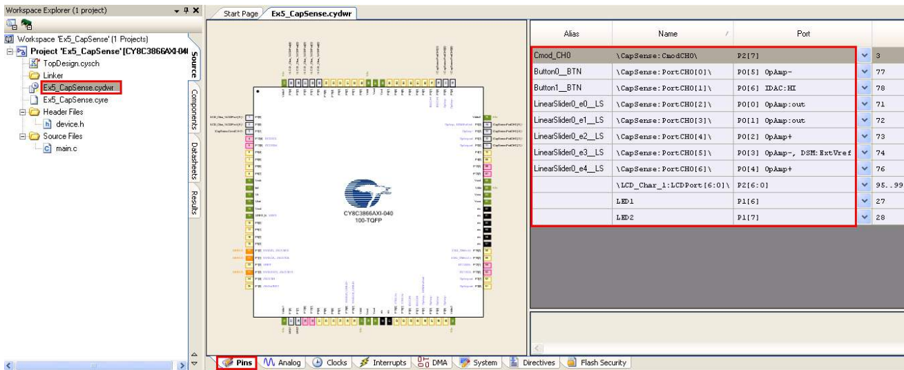
Figure 3-152. Pin Assignment for CY8C38 Family Processor Module
