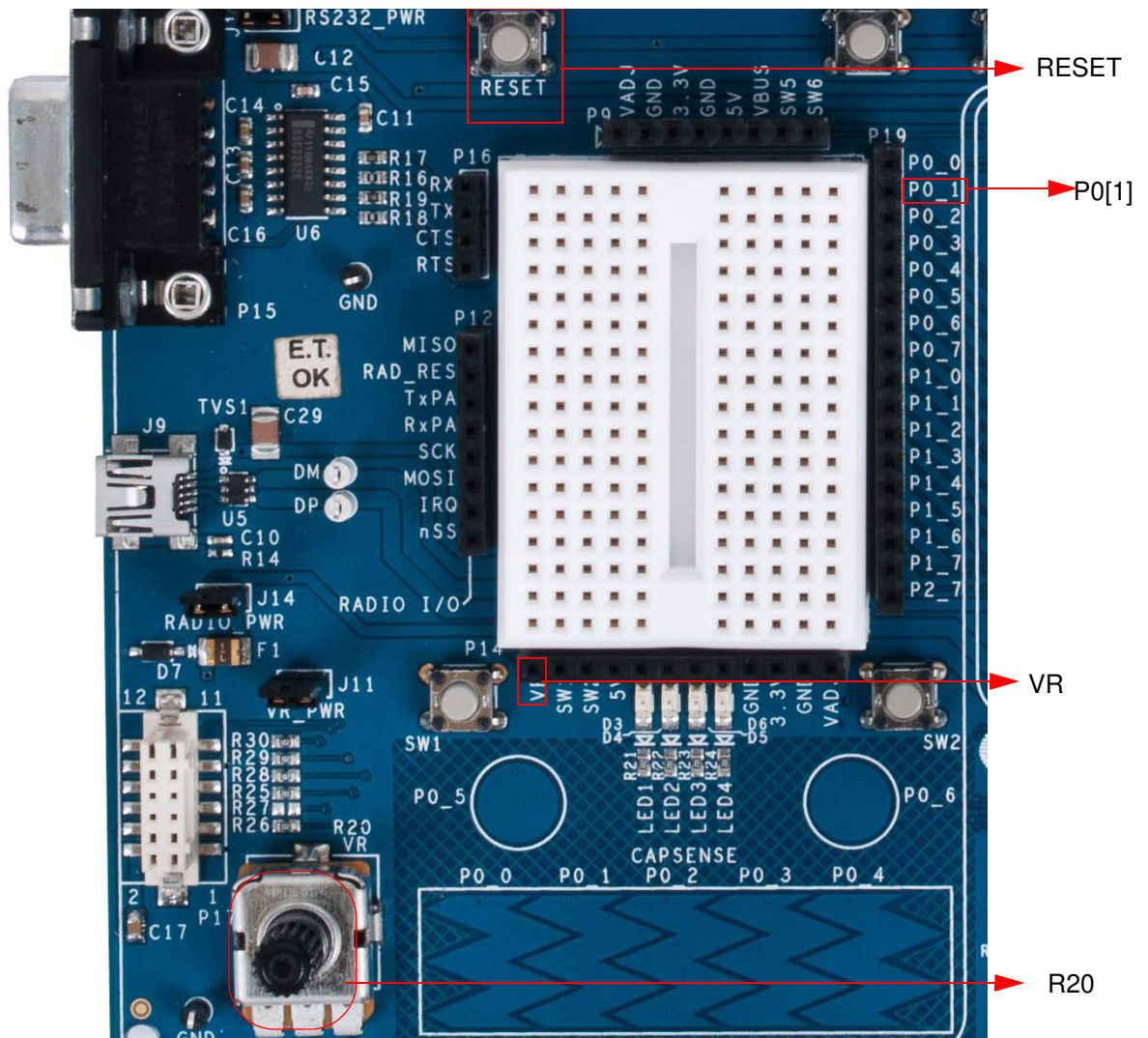
Figure 3-23. Connect P0[1] to VR
