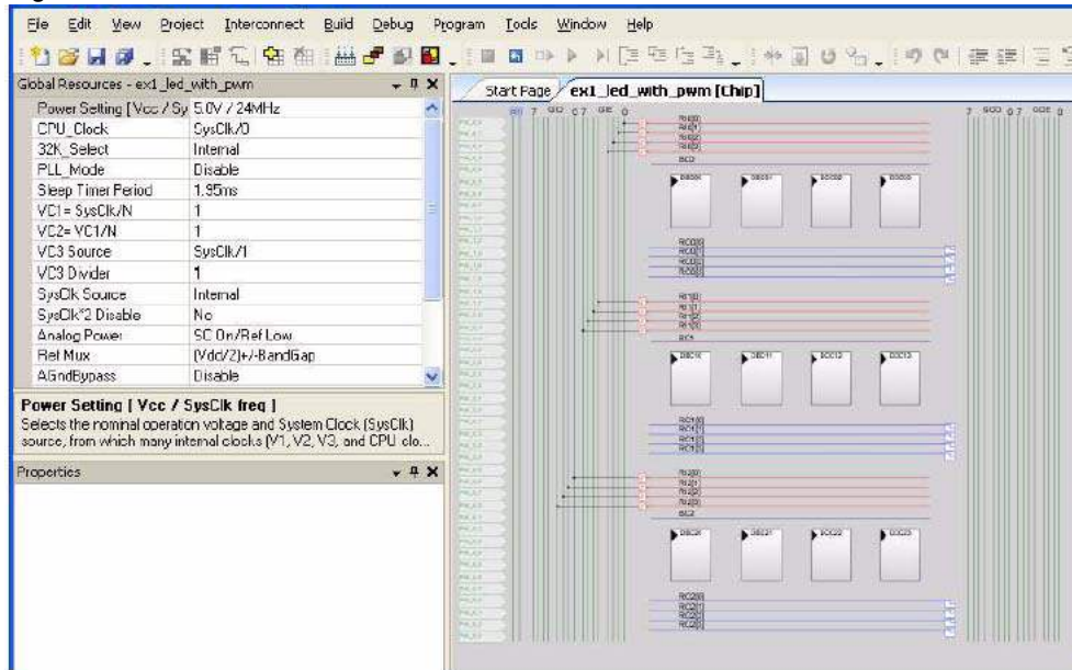
Figure 3-4. Default View.
