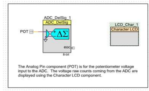
Figure 3-105. Connected Components
