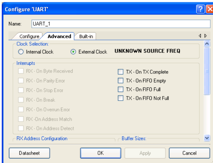
Figure 3-118. Advanced Tab
