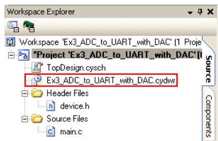
Figure 3-107. Workspace Explorer
