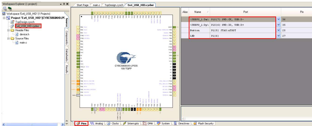
Figure 3-144. Pin Assignments
