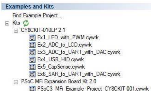
Figure 2-19. Kits List
