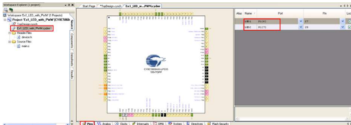
Figure 3-100. Pin Assignments
