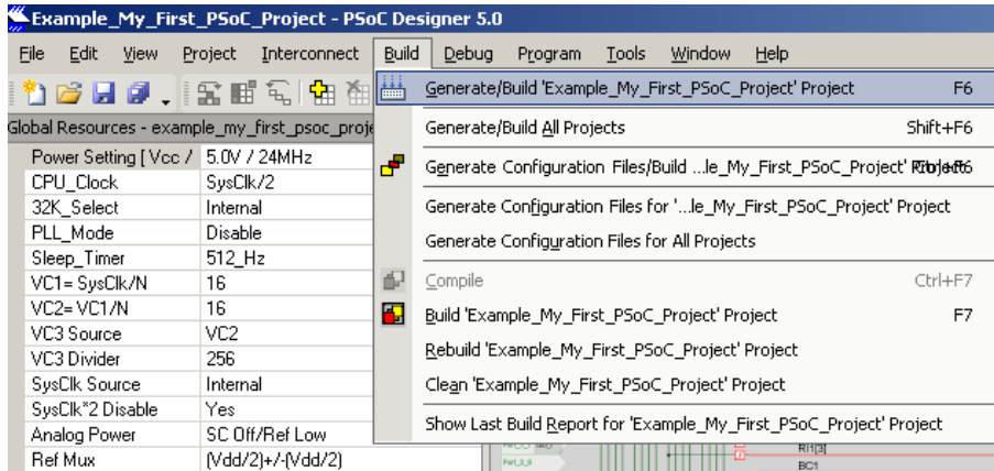
Figure 2-8. Build Project
