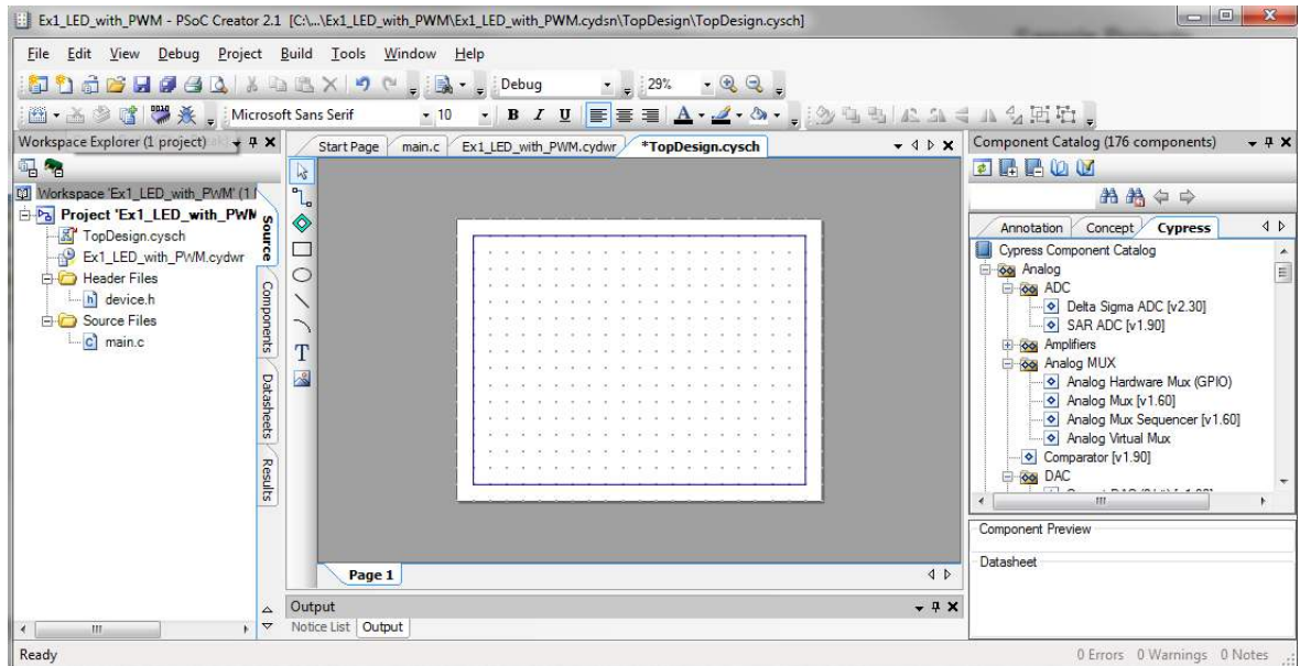
Figure 3-91. Ex1_LED_with_PWM
