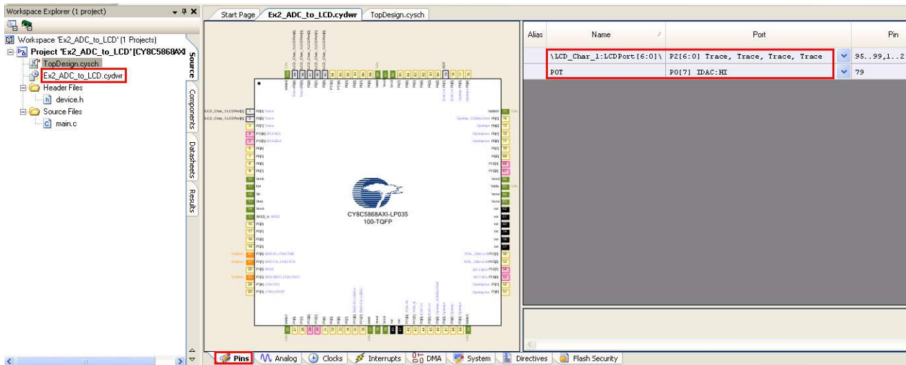
Figure 3-106. Pins Assignments
