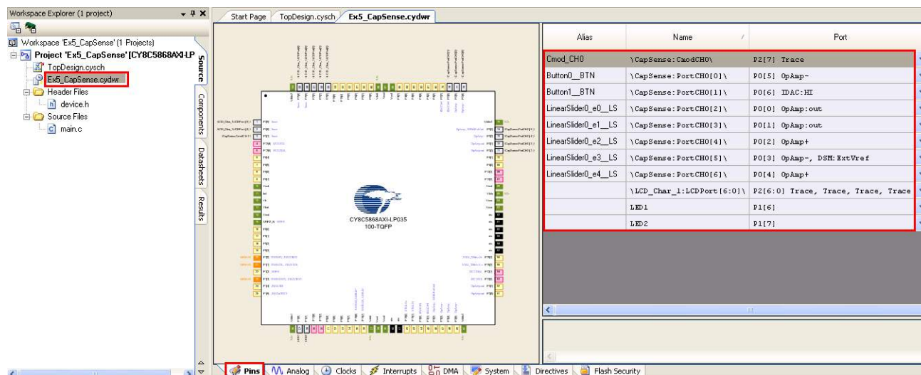
Figure 3-153. Pin Assignment for CY8C58LP Family Processor Module
