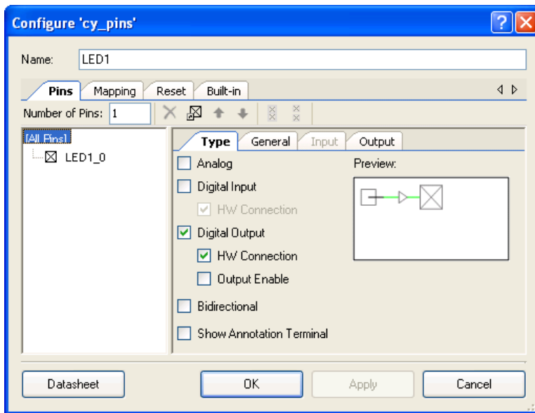
Figure 3-94. LED1 Component Configuration
