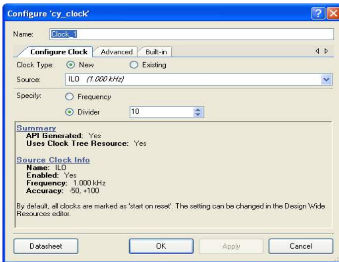
Figure 3-98. Clock Component Configuration
