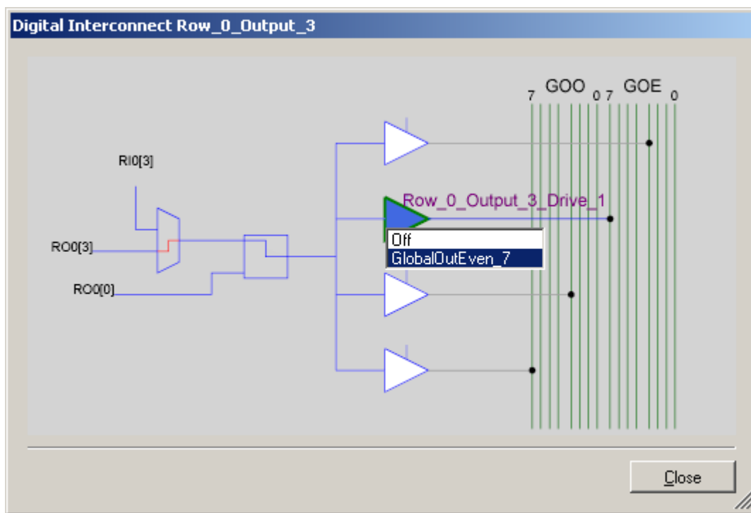
Figure 3-58. Digital Interconnect Window
