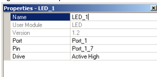
Figure 3-61. Properties Window
