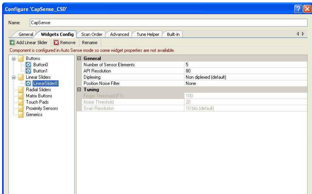
Figure 3-147. Slider Configuration
