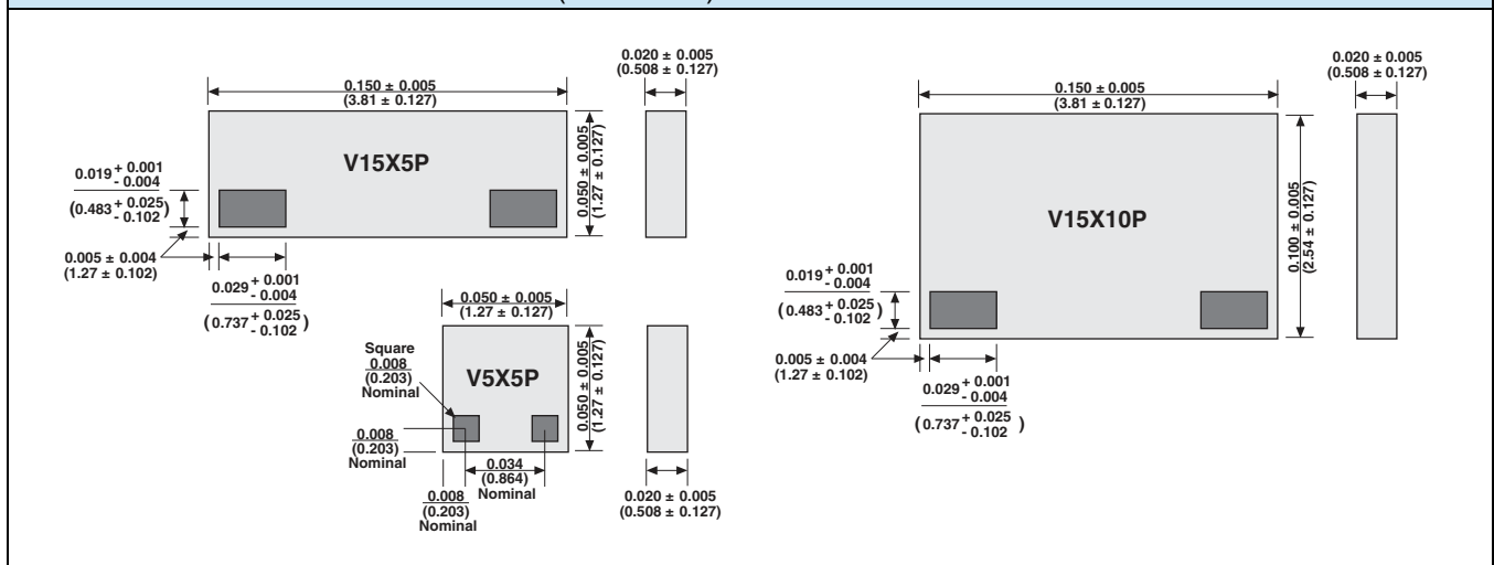
FIGURE 3 - DIMENSIONS in inches (millimeters)
