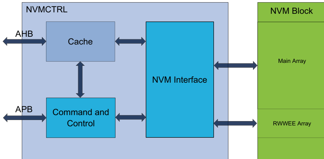
Figure 21-1. Block Diagram
