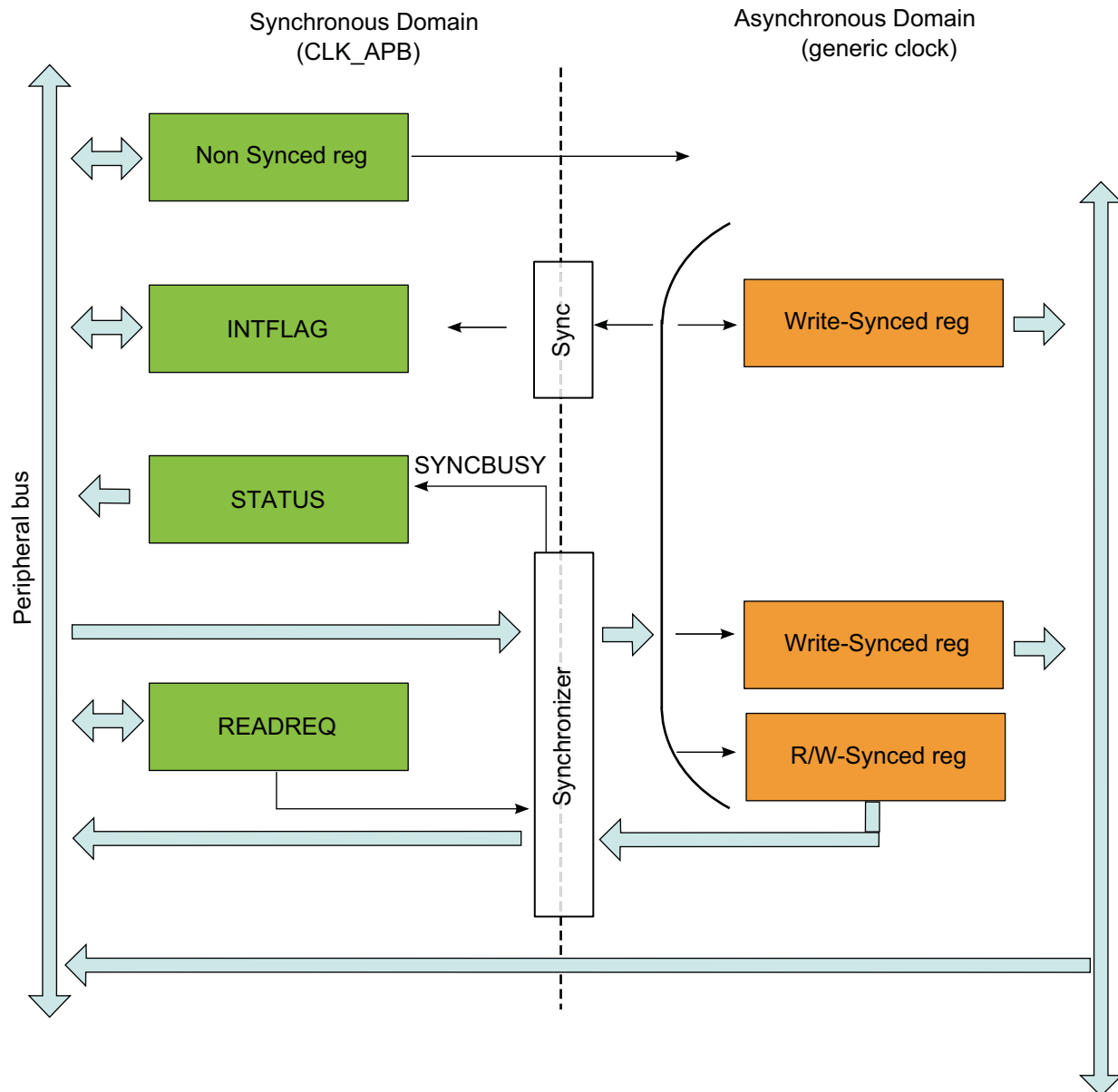
Figure 13-3. Synchronization
