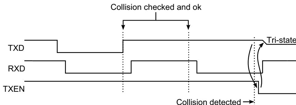
Figure 25-12. Collision Detected
