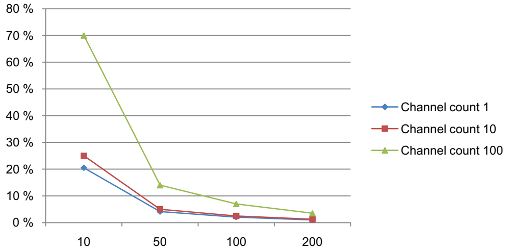
Figure 36-13.CPU Utilization
