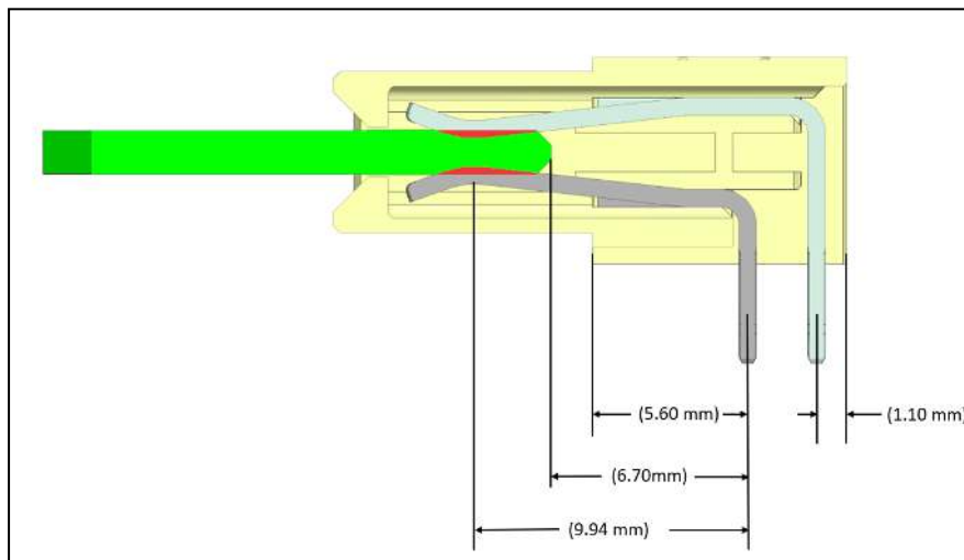
Edge Card mated with Hybrid Right-Angle Receptacle
