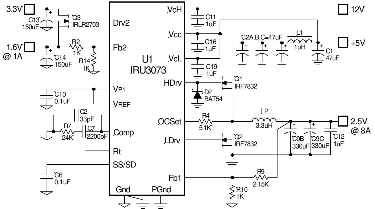
Figure 16 - Typical application of IRU3073.
