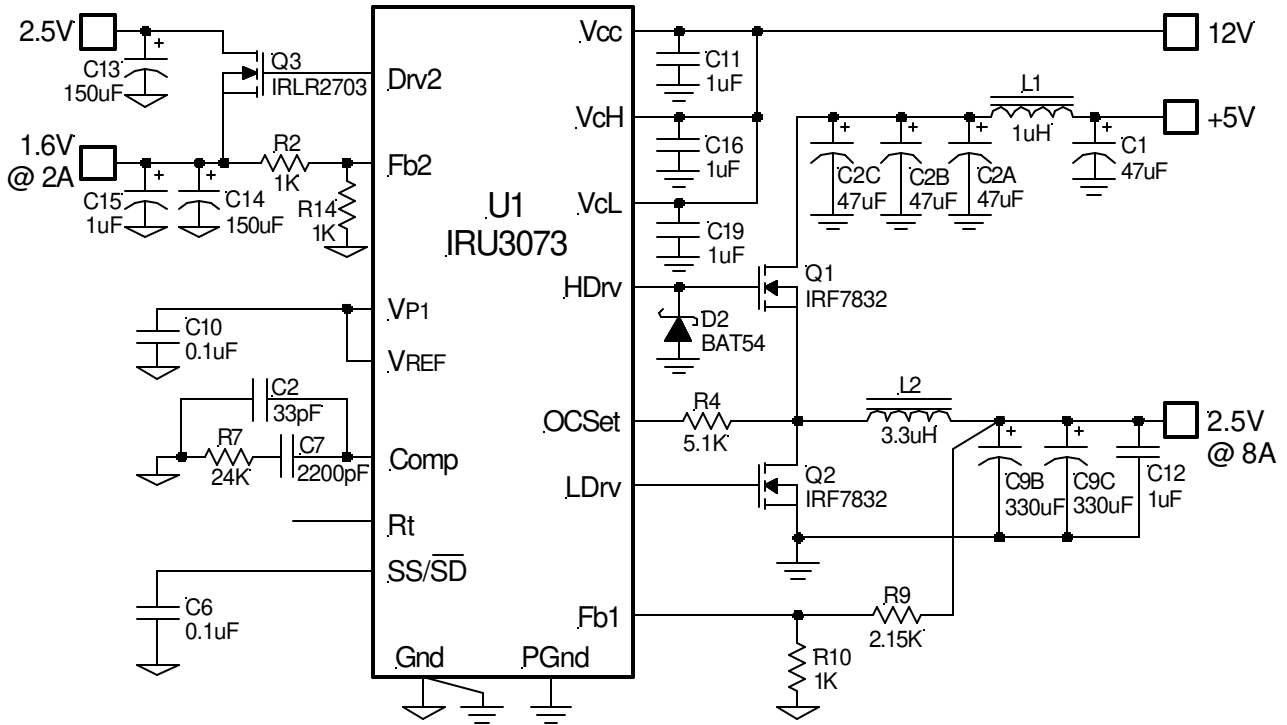
Figure 17 - Typical application of IRU3073.
