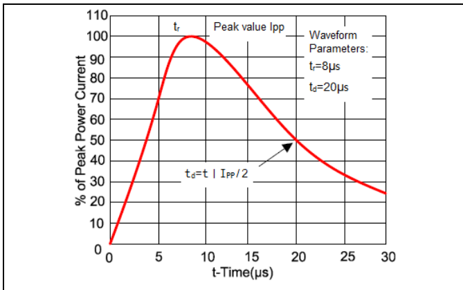
Figure 1. Pulse Waveforms
