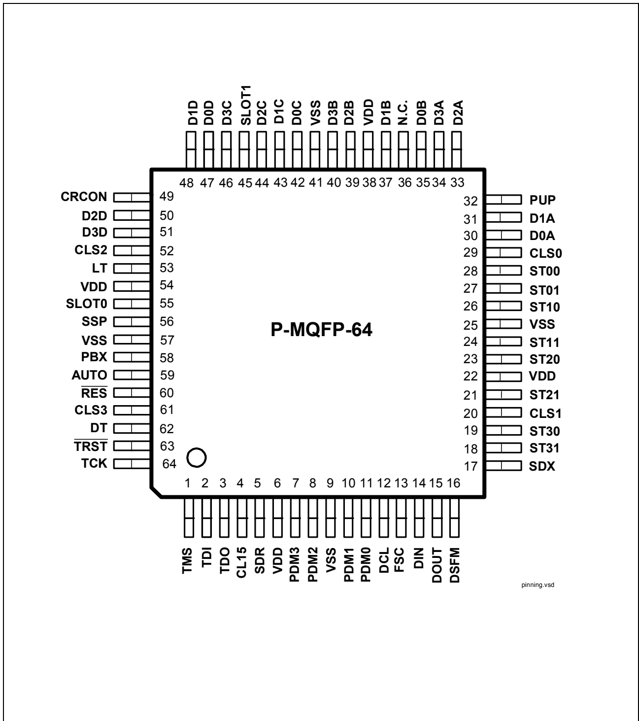
Figure 7 Pin Configuration (63 of 64 used)
