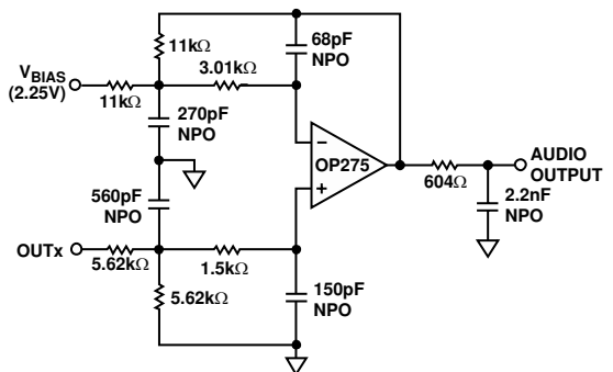
Figure 31. Typical DAC Output Filter Circuit
