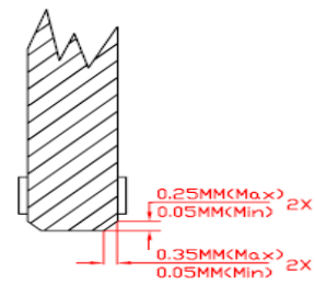
VIEW C-C
