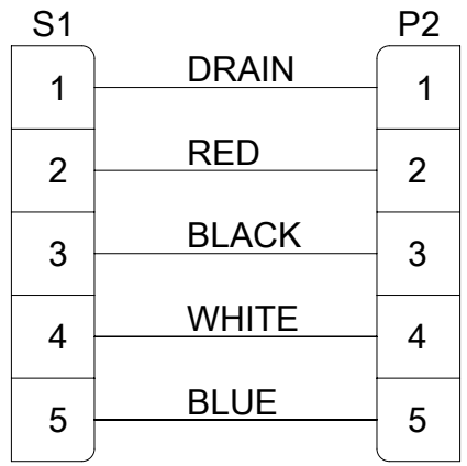
WIRING DIAGRAM
