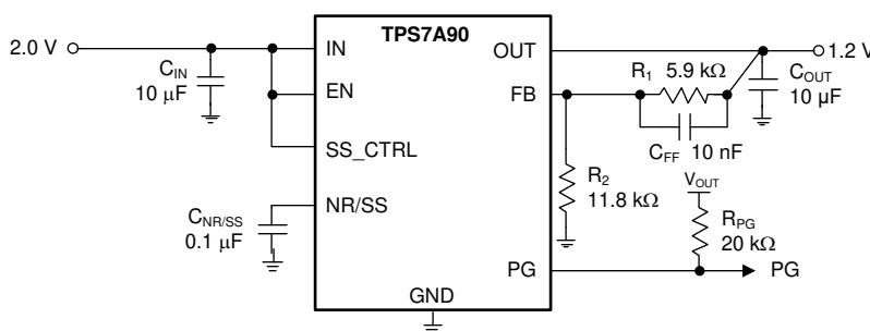
Figure 39. Application Example
