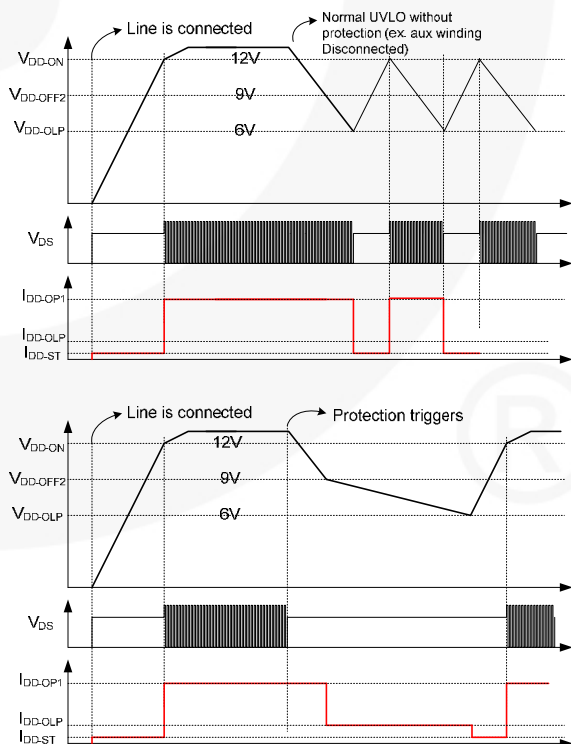
Figure 28. Two-Level UVLO
