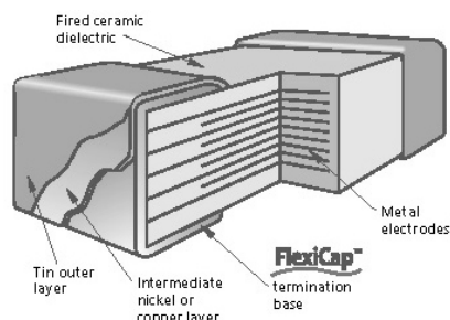
FlexiCap™ MLCC cross section
