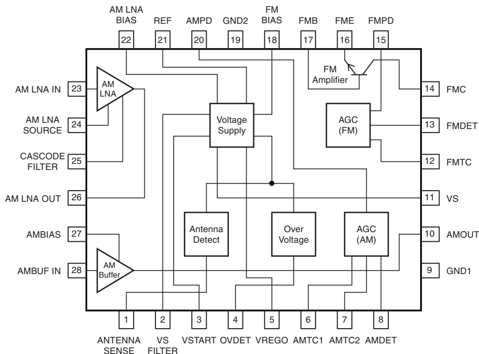
Figure 1-1. Block Diagram
