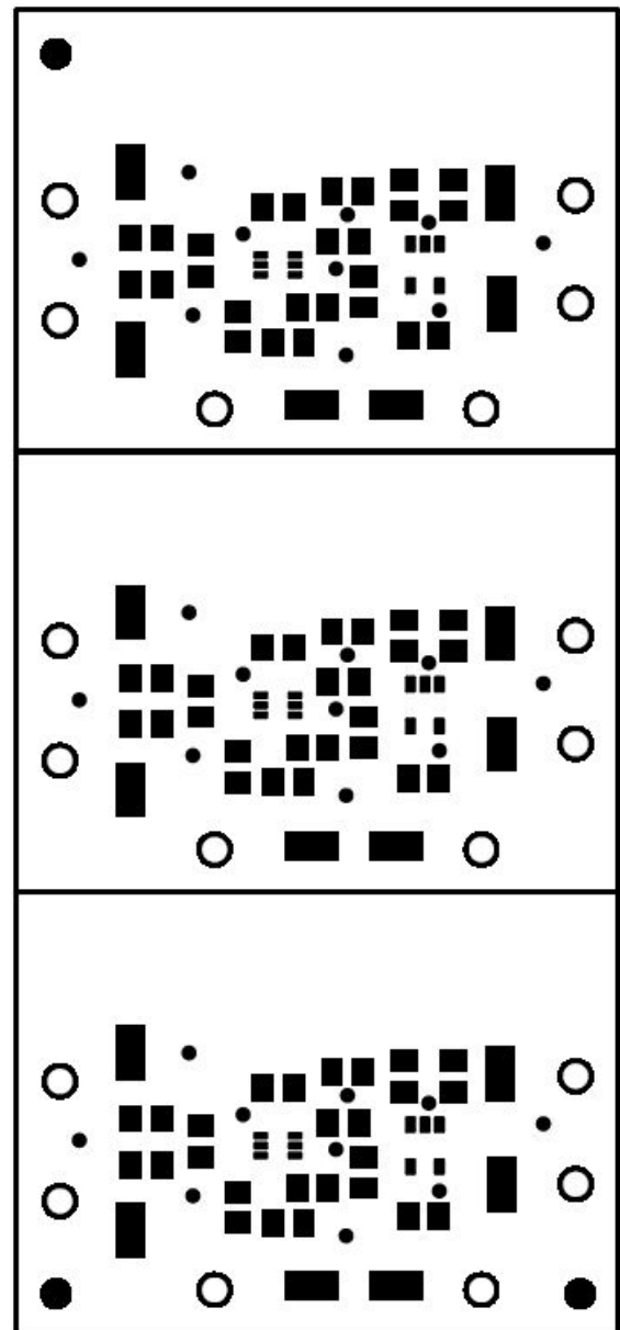
Figure 3. INA199EVM Top Solder Mask
