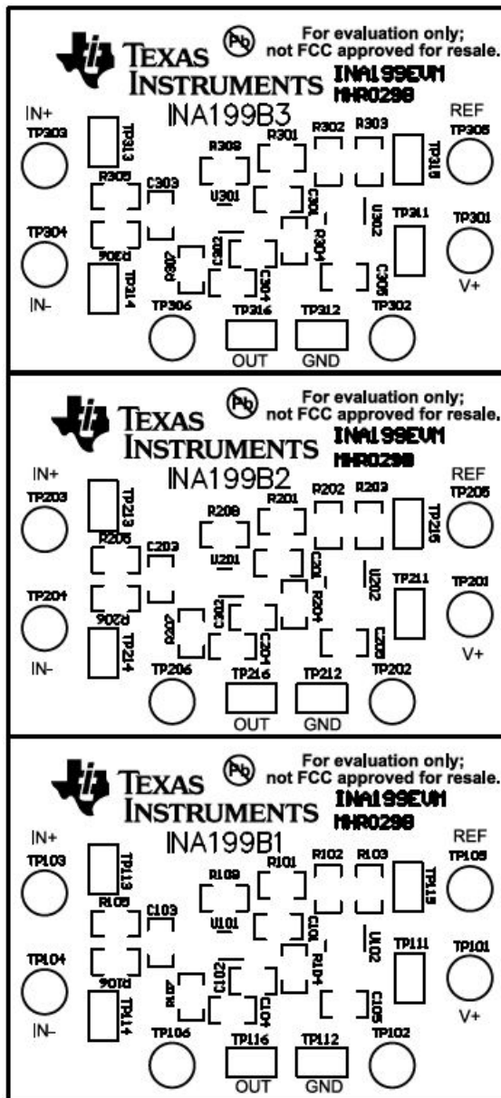
Figure 2. INA199EVM Top Overlay
