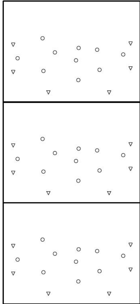
Figure 7. INA199EVM Drill Drawing
