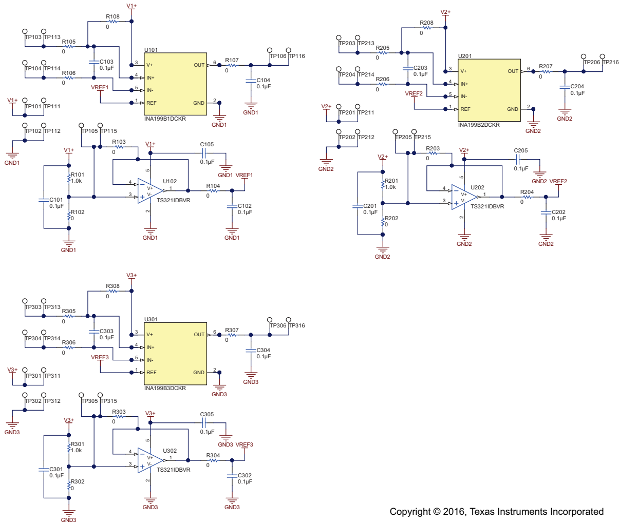
Figure 1. INA199EVM Schematic
