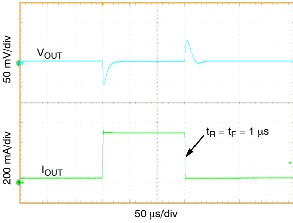
Figure 11. Load Transient Response, I_{OUT} = 50\text{ mA} to 500\text{ mA} , C_{OUT} = 10\text{ }\mu\text{F}
