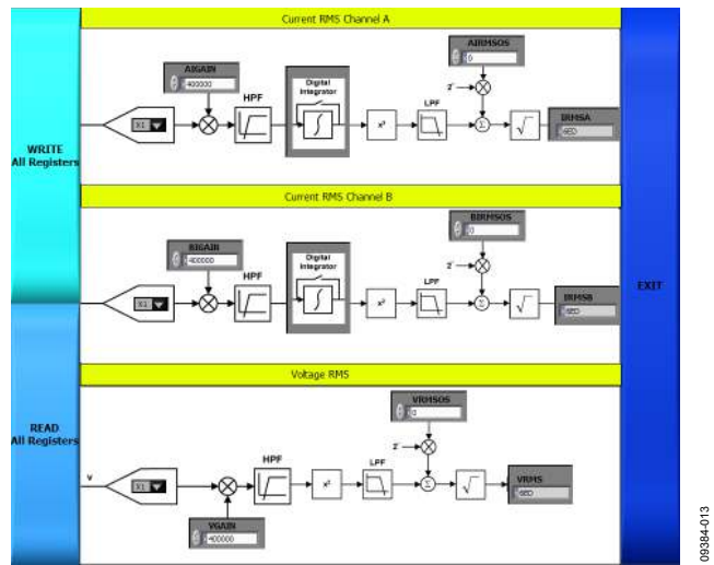
Figure 12. RMS Window
