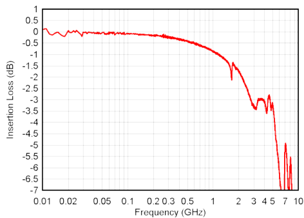
Figure 6-17. Insertion Loss
