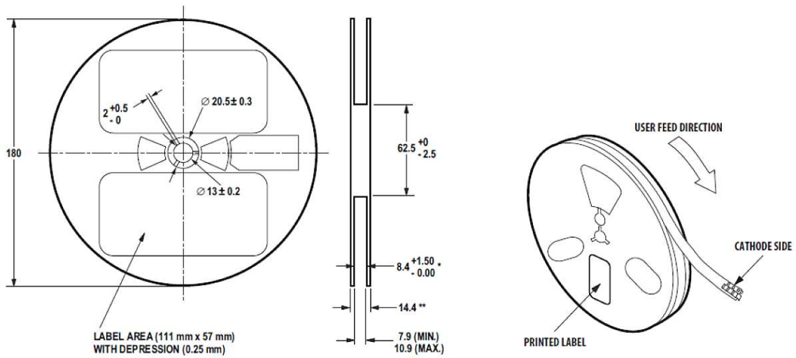
Figure 15: Reel Dimensions
