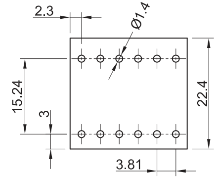
RECOMMENDED PCB LAYOUT - COMPONENT VIEW
