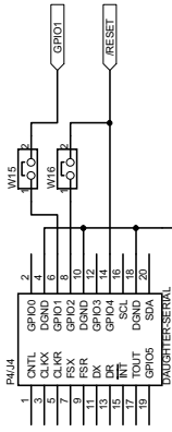
J4 (TOP) = SAMTEC - P/N: TSM-110-01-L-DV-P J4 (BOTTOM) = SAMTEC - P/N: SSW-110-22-F-D-VS
