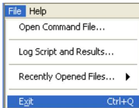
Figure 31. File Menu
