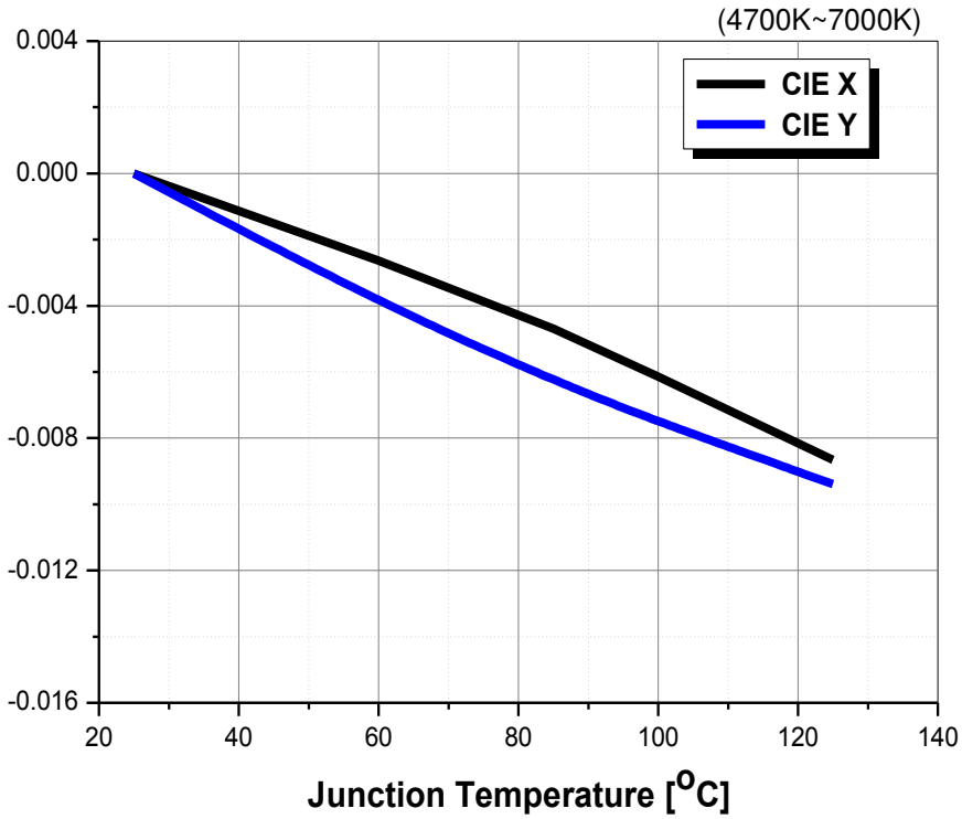
Fig 8. Junction Temp. vs. CIE X, Y Shift, I_F=640mA (CRI80)
