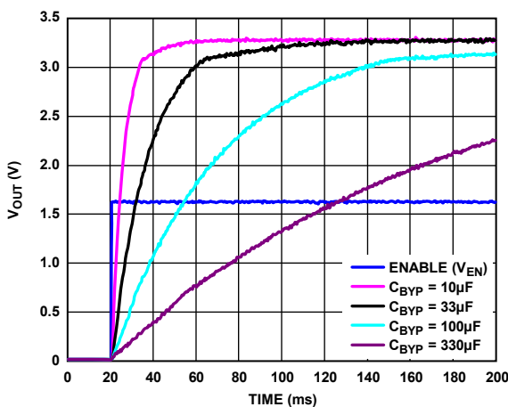
Figure 55. Typical Start-Up Behavior with C_{BYP} = 10 \mu\text{F} to 330 \mu\text{F}
