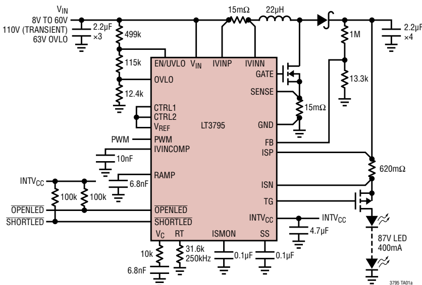
Short-Circuit Robust Boost LED Driver with Spread Spectrum Frequency Modulation
