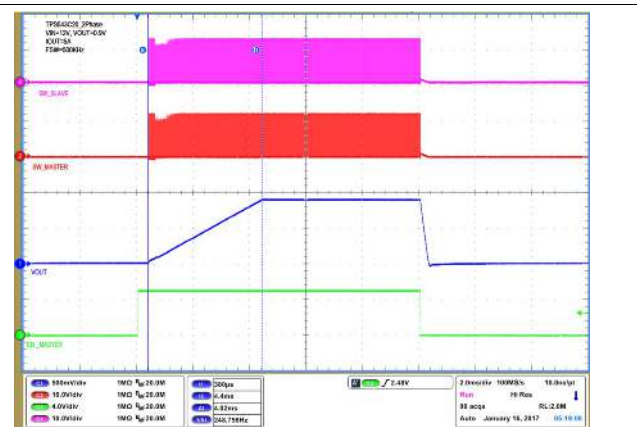
Figure 40. Output Voltage Start-up and Shutdown, 0.9-V Output at 12 VIN, 5-A Output
