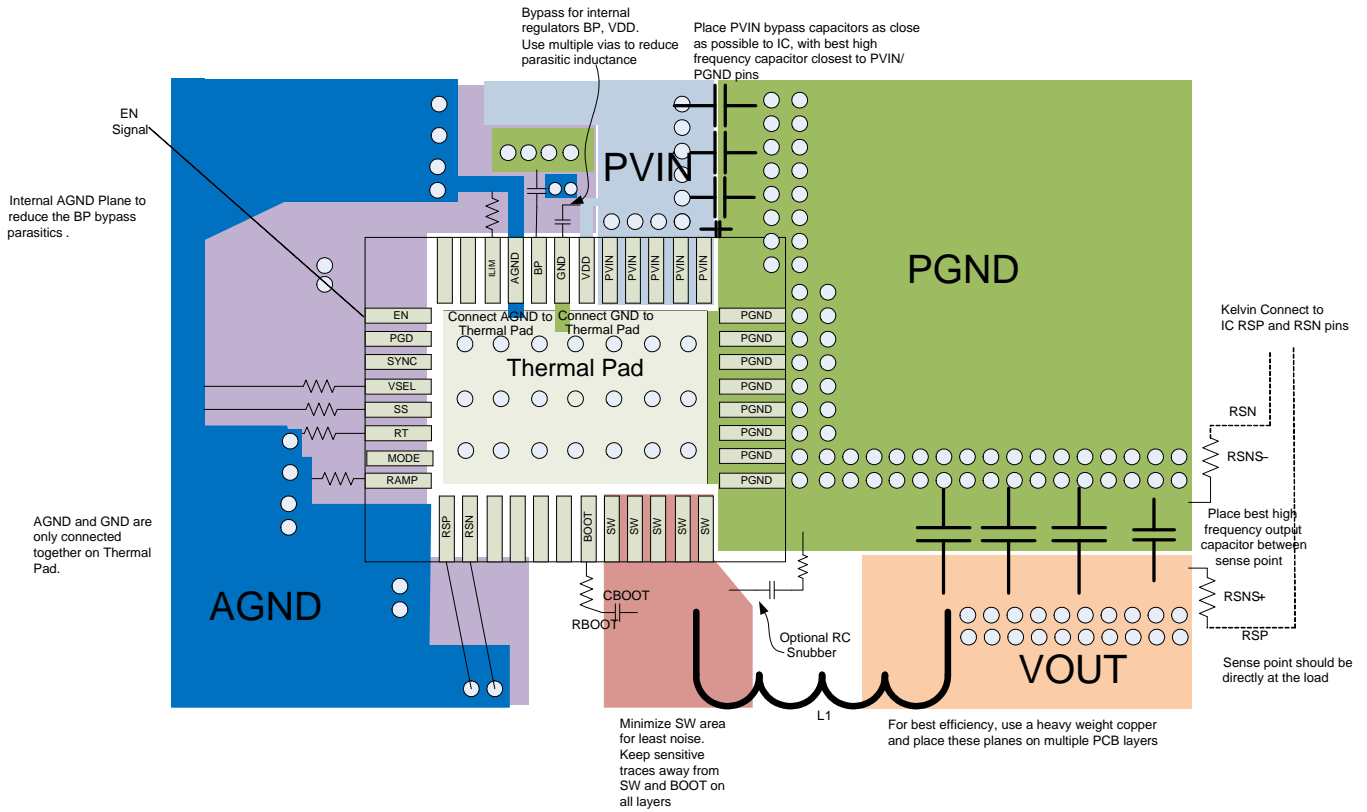
Figure 42. Example Layout
