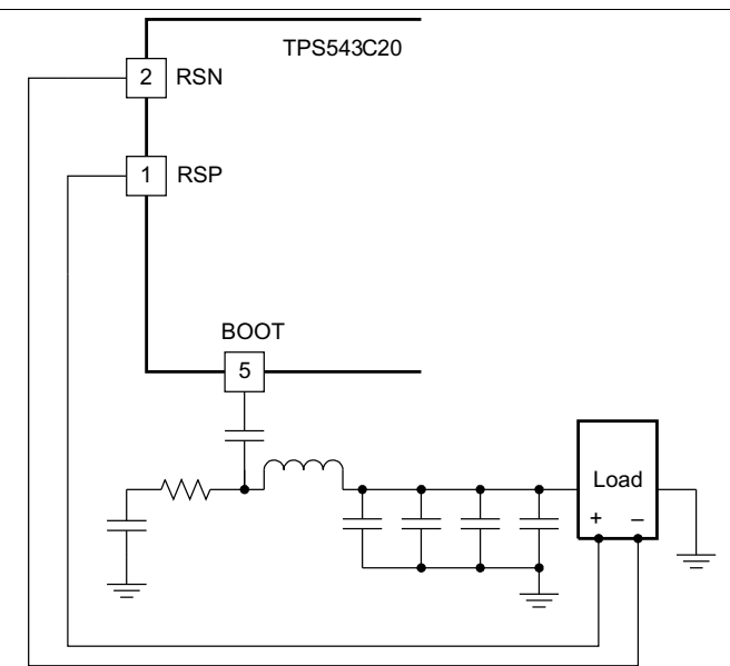
Figure 23. Remote Sensing Without Feedback Resistors
