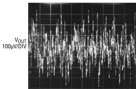
LT1763-5 10Hz to 100kHz Output Noise C_{BYP} = 0
