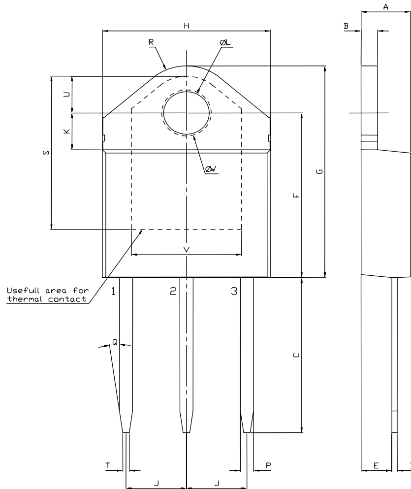
Figure 12. Package outline
