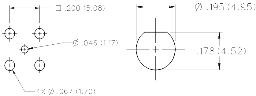
Mounting hole layout
