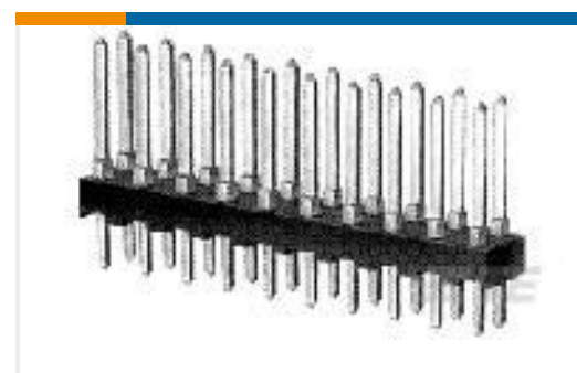
TE Part #1-87227-3 26 MODII HDR DRST UNSHRD .100
