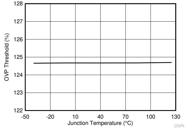
Figure 6-8. OVP Threshold vs Junction Temperature
