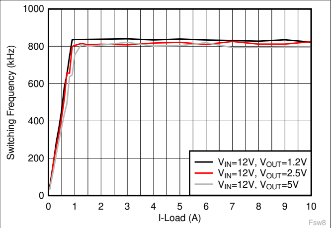
Figure 6-22. Switching Frequency vs Load Current, F_{SW} = 800 kHz, OOA
