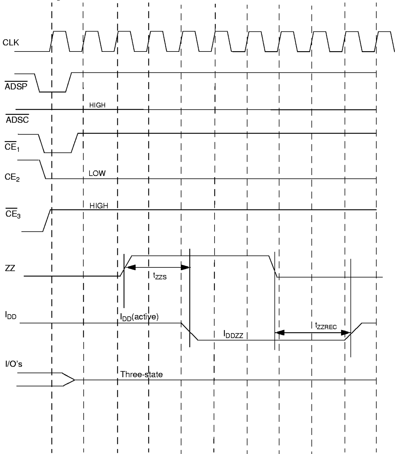
ZZ Mode Timing [19, 20]
