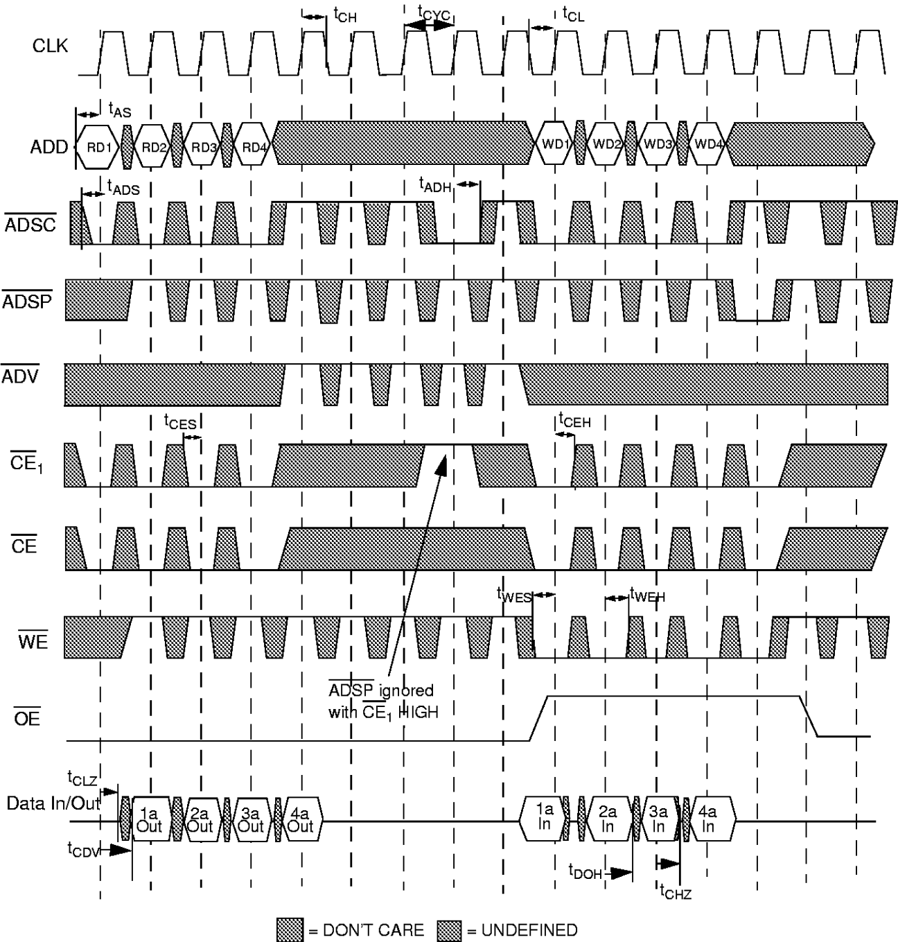
Pipeline Timing (Using \overline{\text{ADSC}} ) [17, 18]
