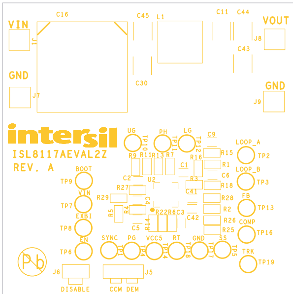
FIGURE 7. SILKSCREEN TOP
