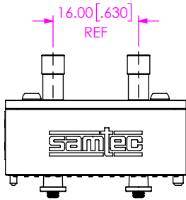
FIG 5 BE40A-S-XXXX-X-2-08-XXXX SHOWN CABLE ASSEMBLIES NOT SHOWN FOR CLARITY
