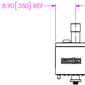
FIG 8 BE40A-S-XXXX-X-2-03-XXXX SHOWN CABLE ASSEMBLIES NOT SHOWN FOR CLARITY
