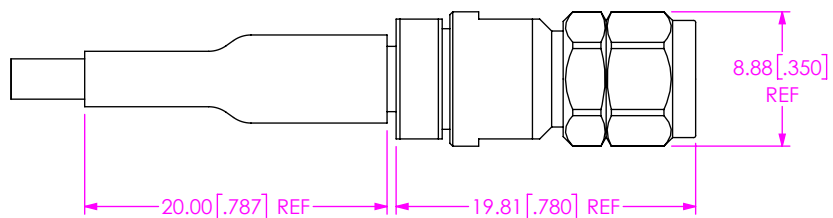
FIG 11 -24SP SHOWN
