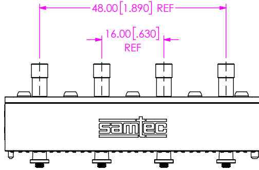
FIG 2 BE40A-S-XXXX-X-2-16-XXXX SHOWN CABLE ASSEMBLIES NOT SHOWN FOR CLARITY
