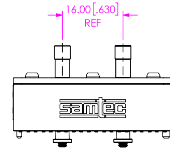
FIG 4 BE40A-S-XXXX-X-2-10-XXXX SHOWN CABLE ASSEMBLIES NOT SHOWN FOR CLARITY
