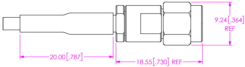
FIG 9 -92SP SHOWN
