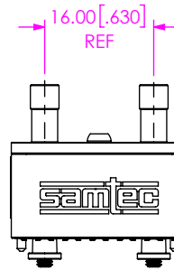
FIG 6 BE40A-S-XXXX-X-2-06-XXXX SHOWN CABLE ASSEMBLIES NOT SHOWN FOR CLARITY
