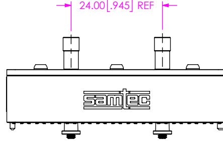
FIG 3 BE40A-S-XXXX-X-2-14-XXXX SHOWN CABLE ASSEMBLIES NOT SHOWN FOR CLARITY
