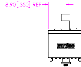
FIG 7 BE40A-S-XXXX-X-2-04-XXXX SHOWN CABLE ASSEMBLIES NOT SHOWN FOR CLARITY
