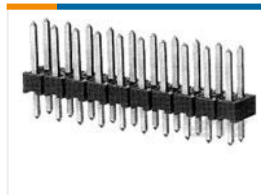
TE Part #5-146257-8 16 MODII HDR DRST B/A .100CL L
