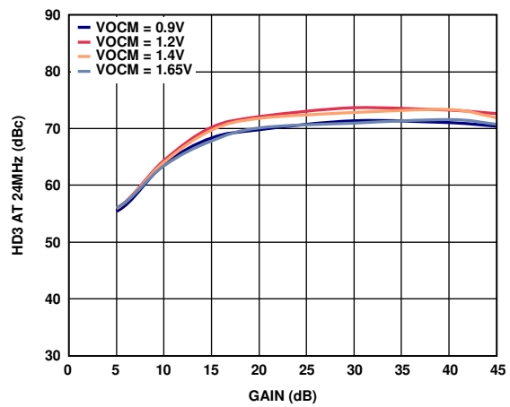
Figure 22. HD3 vs. Gain over Output Common-Mode Voltage (Bandwidth Setting = 31 MHz, 1.5 V p-p, 8 MHz CW Fundamental Output)
