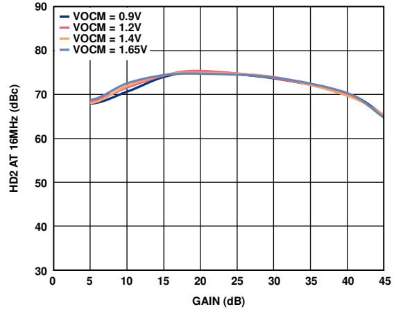
Figure 20. HD2 vs. Gain over Output Common-Mode Voltage (Bandwidth Setting = 31 MHz, 1.5 V p-p, 8 MHz CW Fundamental Output)
