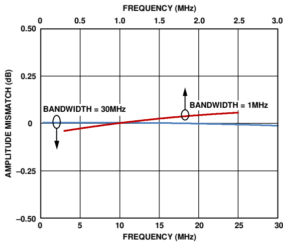
Figure 18. IQ Amplitude Matching vs. Frequency
