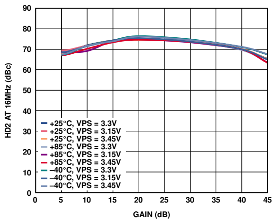
Figure 19. HD2 vs. Gain over Supply and Temperature (Bandwidth Setting = 31 MHz, 1.5 V p-p, 8 MHz CW Fundamental Output)
