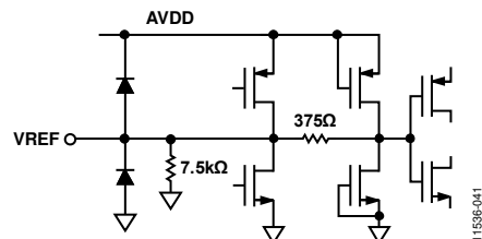
Figure 31. Equivalent VREF Circuit
