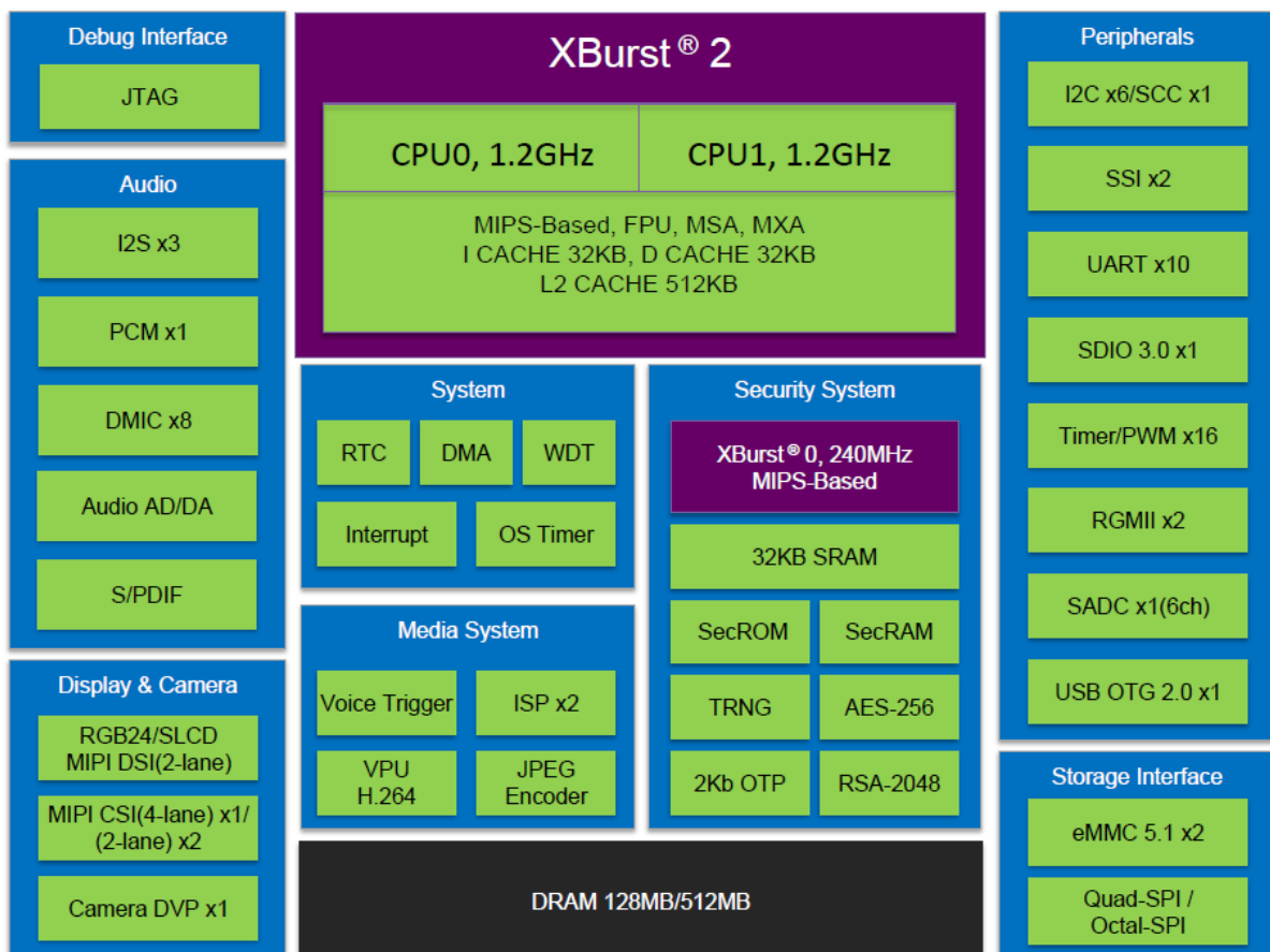
Figure 1-1 X2000 Diagram
