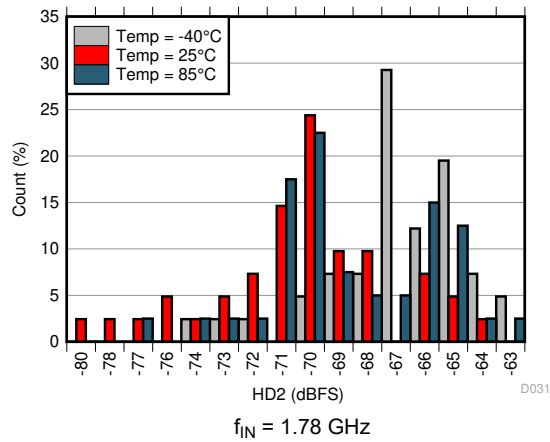
f_{IN} = 1.78 \text{ GHz} Figure 6-55. HD2 Histogram at AVDD19 = 1.8 V
