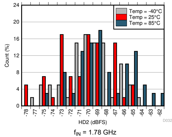
f_{IN} = 1.78 \text{ GHz} Figure 6-56. HD2 Histogram at AVDD19 = 1.9 V
