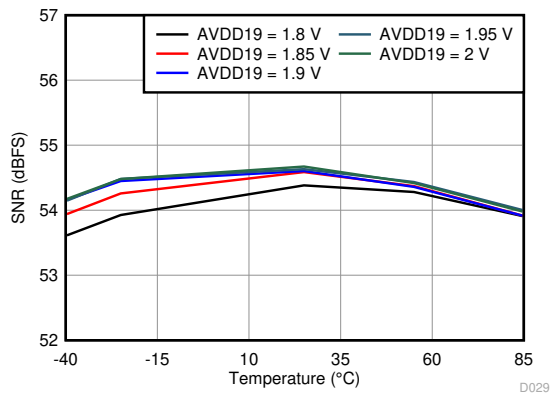
f_{IN} = 3.5 \text{ GHz} , A_{IN} = -3 \text{ dBFS} with 2-dB digital gain Figure 6-53. Signal-to-Noise Ratio vs. AVDD19 Supply and Temperature
