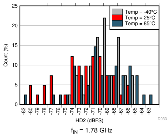
f_{IN} = 1.78 \text{ GHz} Figure 6-57. HD2 Histogram at AVDD19 = 2.0 V
