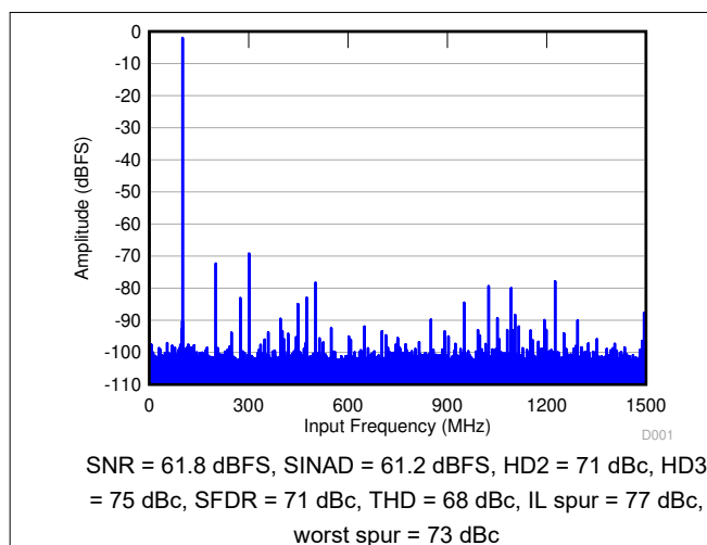
Figure 9-11. FFT for 100-MHz Input Frequency
