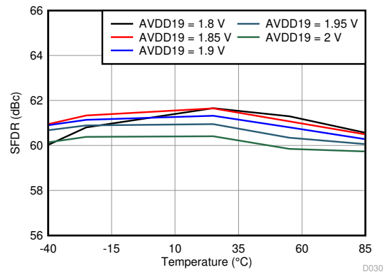
f_{IN} = 3.5 \text{ GHz} , A_{IN} = -3 \text{ dBFS} with 2-dB digital gain Figure 6-54. Spurious-Free Dynamic Range vs. AVDD19 Supply and Temperature
