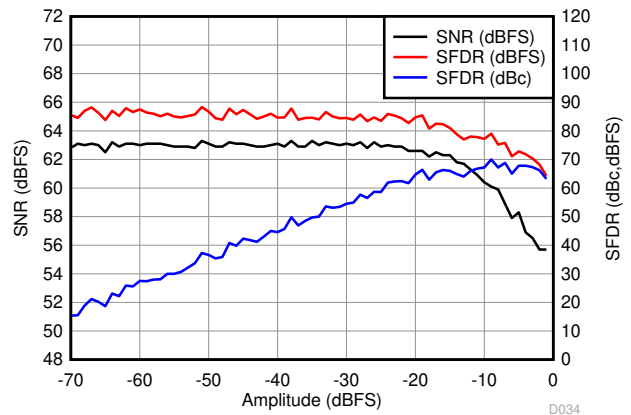
f_{IN} = 1.78 \text{ GHz} , A_{IN} = -2 \text{ dBFS} Figure 6-58. Performance vs. Amplitude
