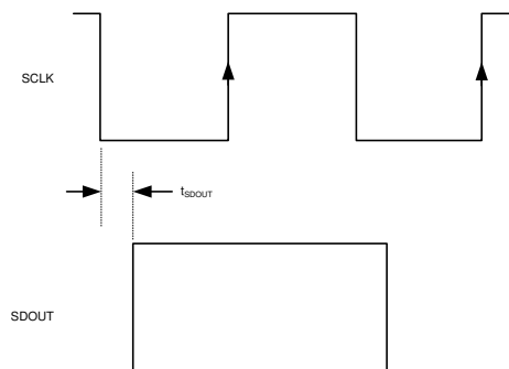
Figure 8-57. SDOOUT Timing
