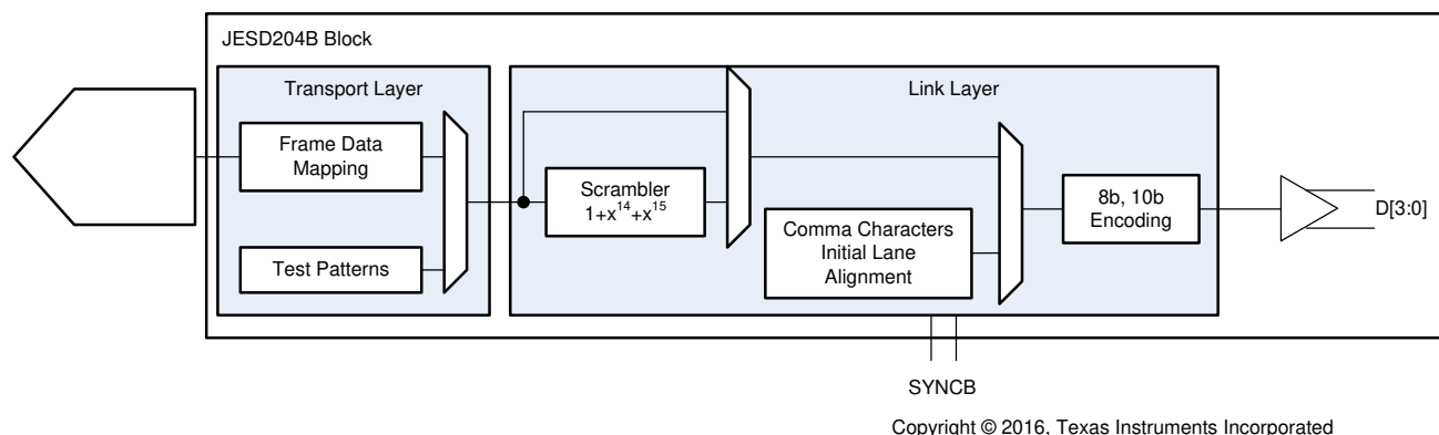
Figure 8-54. JESD Digital Block Implementation
