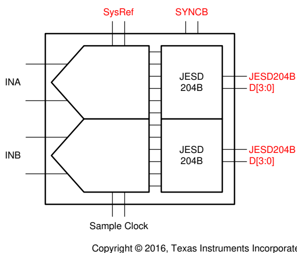
Figure 8-53. JESD Signal Overview
