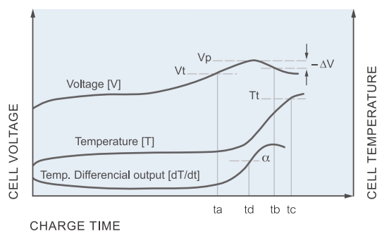
FIG. 24 Charging characteristics (Charging current > 0.5 CA)
