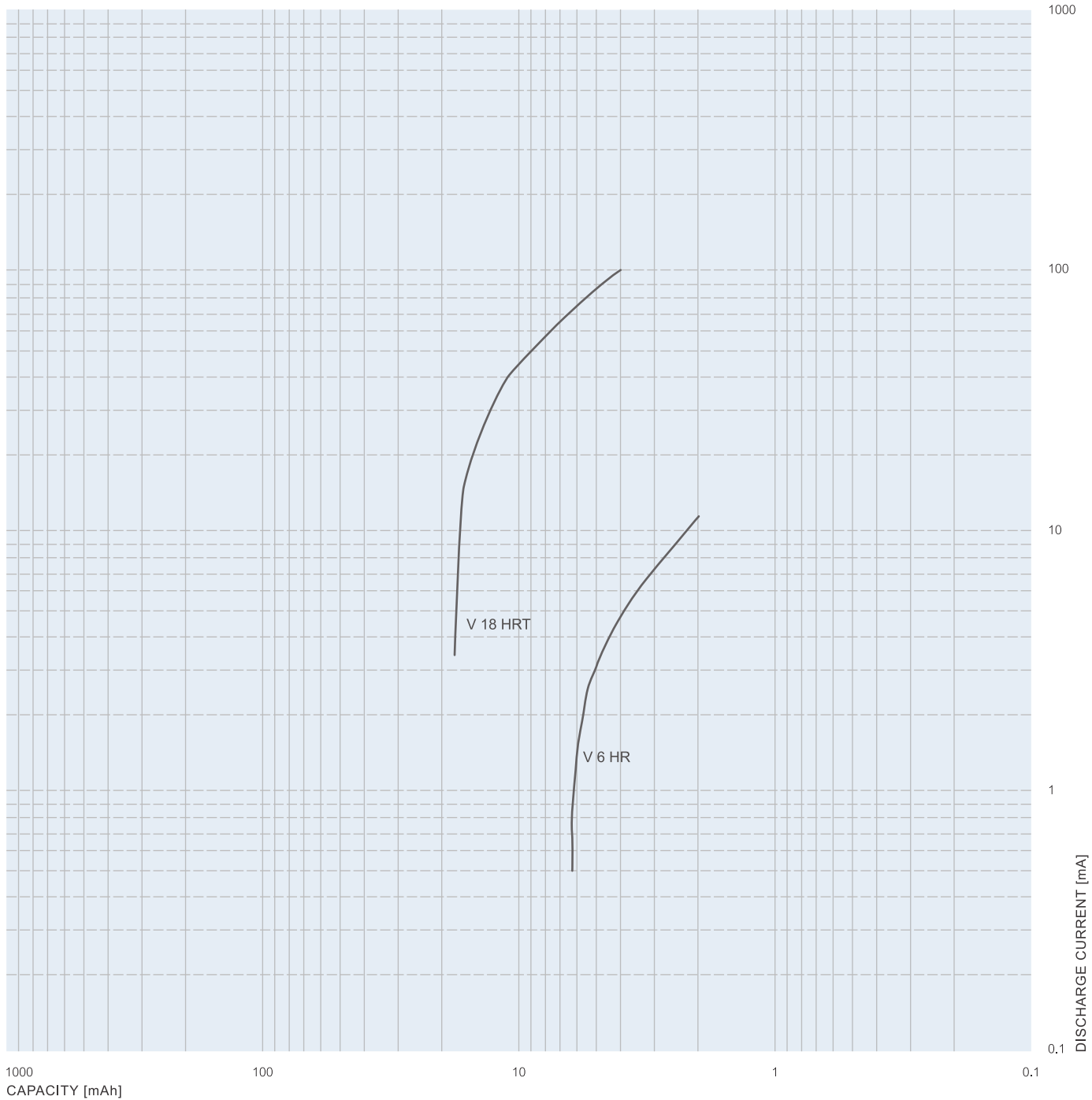
FIG. 36 Discharge characteristics V 18 HRT, V 6 HR
