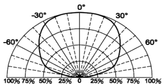
Fig.6 Directivity Radiation
