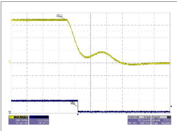
Figure 29. Over-voltage protection, VOUT = 1.5 V
