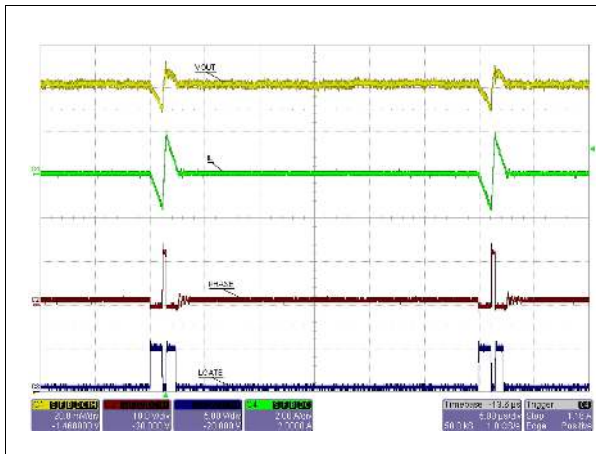
Figure 17. No-audible pulse-skip waveforms
