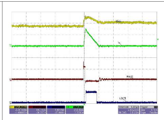
Figure 18. Pulse-skip waveforms
