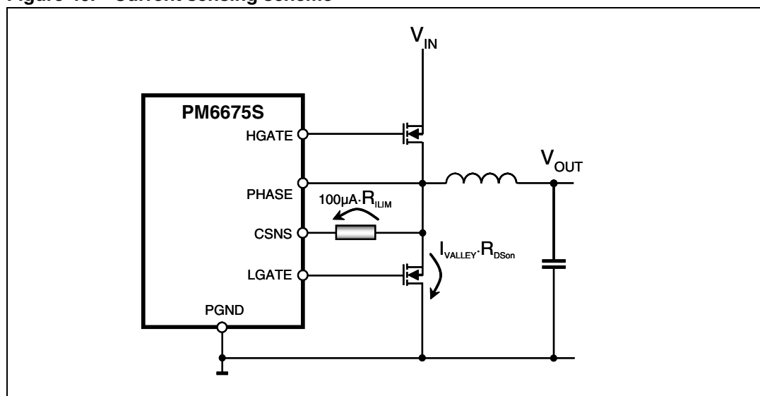
Figure 40. Current sensing scheme
