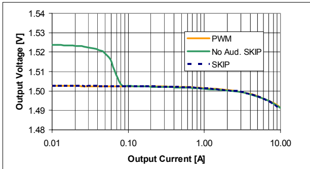
Figure 5. VOUT load regulation, 1.5 V, Vin = 12 V
