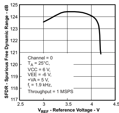
Figure 50. Spurious Free Dynamic Range vs Reference Voltage
