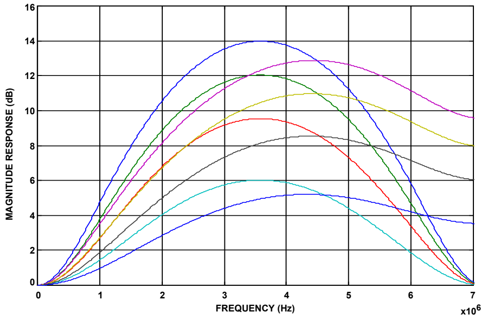
FIGURE 7. CHARACTERISTICS OF THE PEAKING FILTER
