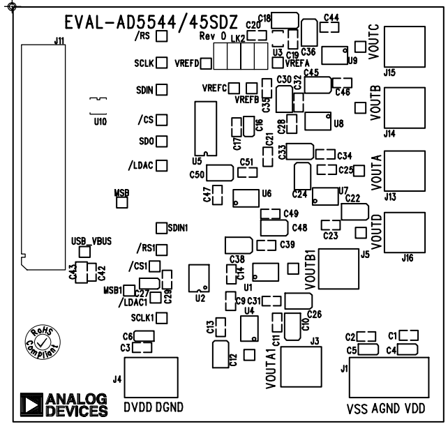
Figure 30. Silkscreen
