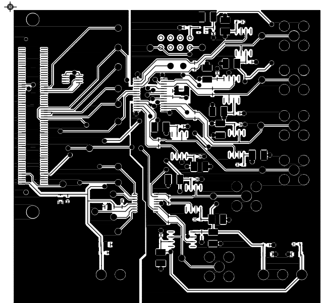
Figure 31. Component Side
